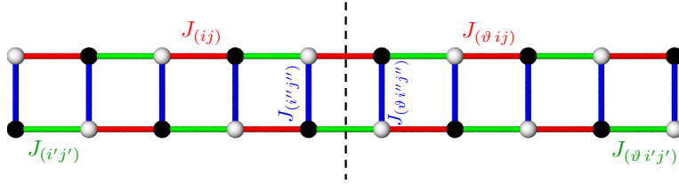
Fig. 3. Case II: Vertical reflection plane. Recall that J_{(ij)} = J_{(ji)} .
