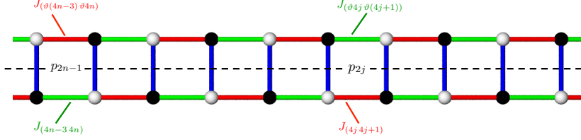
Fig. 2. Case I: Horizontal reflection plane for an open or closed ladder.
