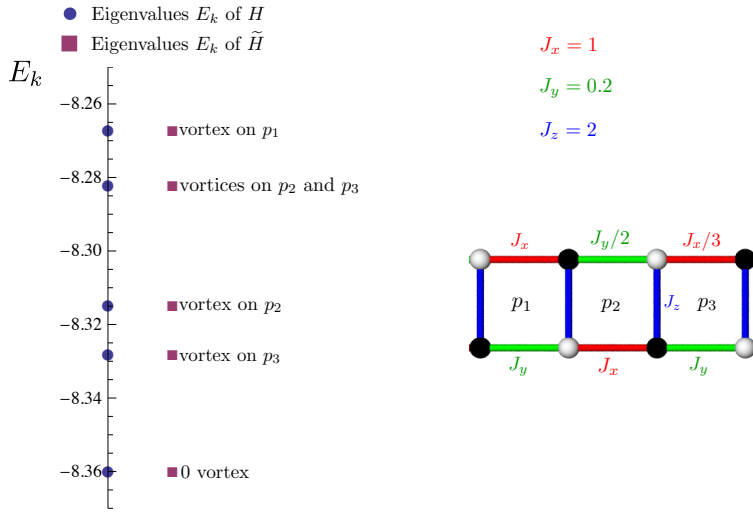
Fig. 5. Low-lying eigenvalues of H and \tilde{H} for an open ladder with the illustrated couplings. We plot eigenvalues of H with circles and those of \tilde{H} with squares, and we ignore multiplicities. Other couplings yield qualitatively similar plots.
