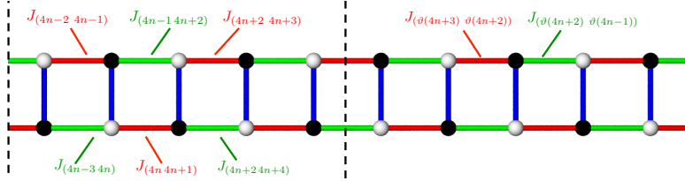
Fig. 4. Case III: Vertical reflection of a closed ladder.
