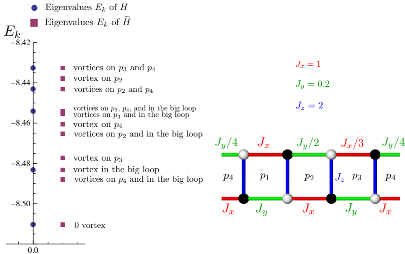
Fig. 7. Low-lying eigenvalues of H and \tilde{H} for an N = 2 closed ladder without symmetry. Here \tilde{H} has eigenvalues that do not occur in H . We refer to the “big loop” as a loop with four horizontal bonds (around either the top or the bottom of the ladder). As in Fig. 5 we ignore multiplicities.
