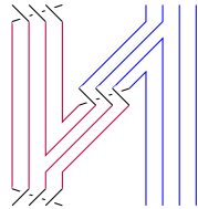
2D projection of CNOT
