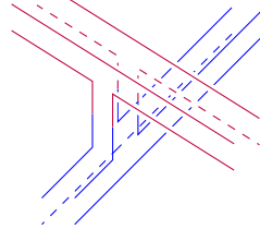
3D CNOT
