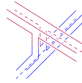
Quon CNOT
