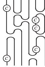
FIGURE 4. A regular planar 6-tangle labelled by c
