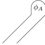
FIGURE 1. Holographic protocol for teleportation of qudit \phi_A .
