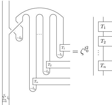
FIGURE 2. CT Protocol for teleportation of compressed transformations.
